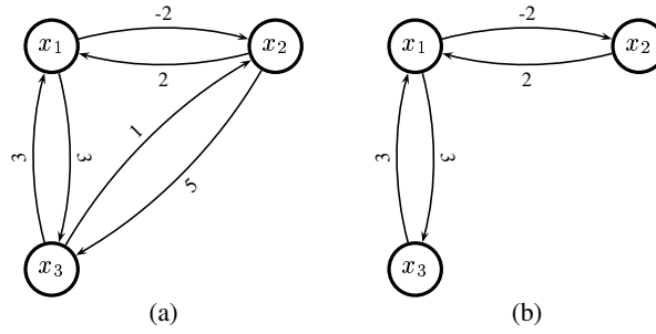
Fig. 10. A graph with a zero-cycle and its minimal form
